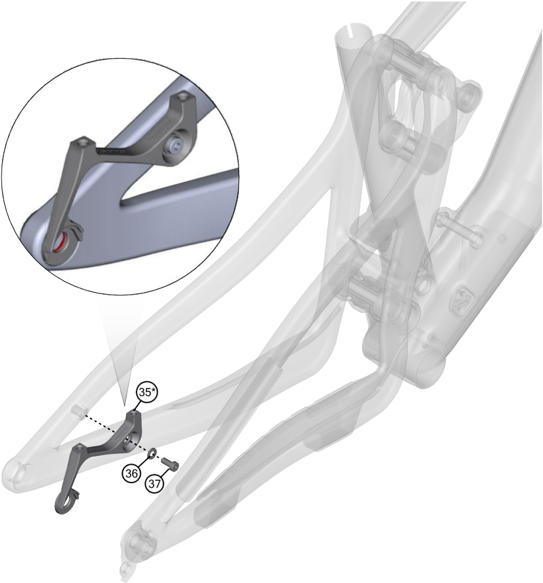
BRAKE MOUNT KIT RIOT CF/PATH RIOT - KE0358
